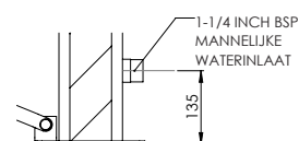
DETAIL C SCHAAL 1: 10
